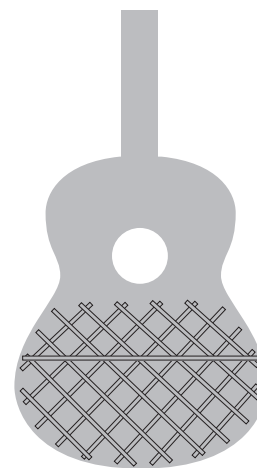
Lattice
